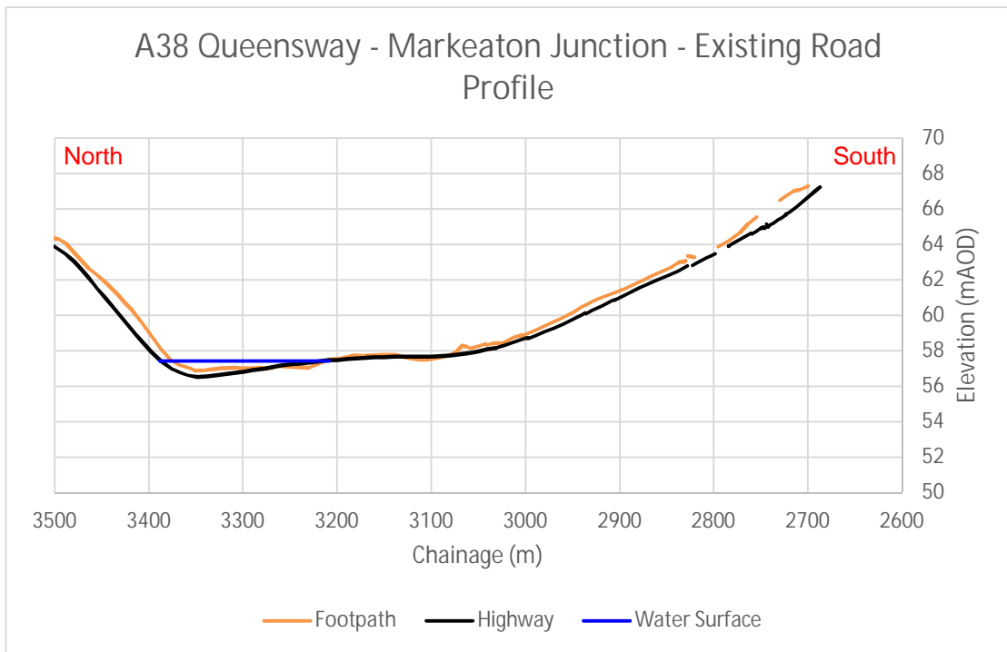
Figure 4-3: Existing road profile along A38 Markeaton showing approximate maximum surface water level in 1% AEP plus 40% climate change event
